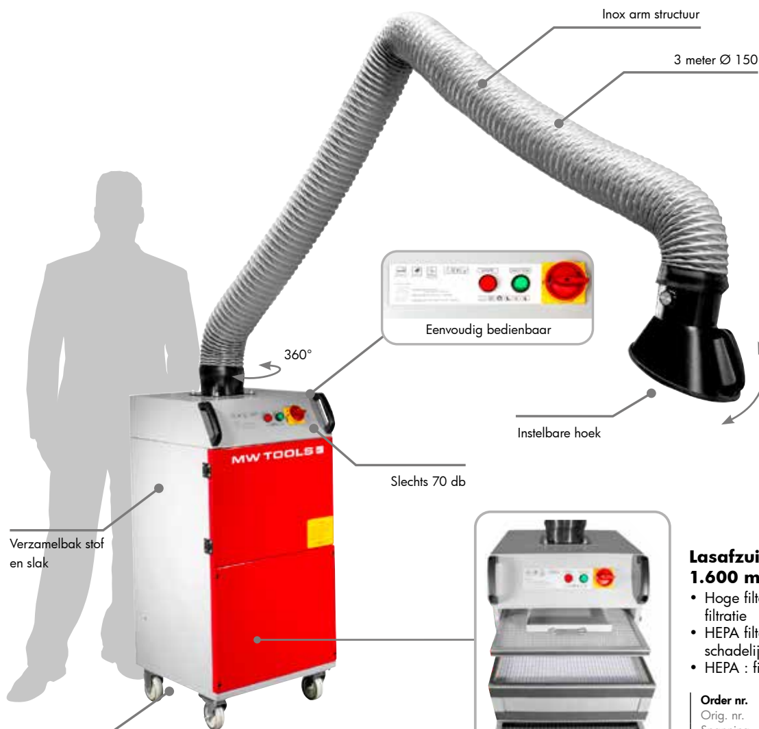
3 traps filter
